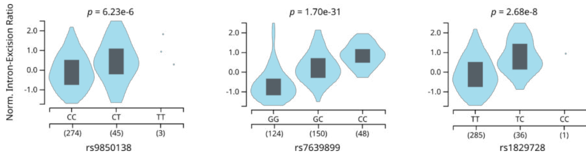
Figure S2. The violin plots of rs9850138, rs7639899, and rs1829728 splicing quantitative trait loci (sQTL) results obtained from the Genotype-Tissue Expression (GTEx) project.
