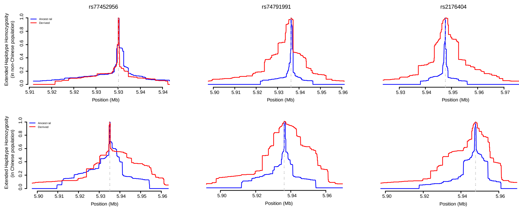
Figure S4. EHH analysis results of rs77452956, rs74791991, and rs2176404, respectively. The lower and upper panels show results from Chinese and non-Chinese populations, respectively.
