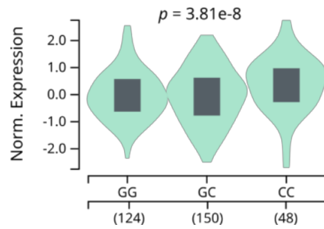
Figure S3. The violin plots of rs7639899 expression quantitative trait loci (mQTL) result obtained from the GTEx project.
