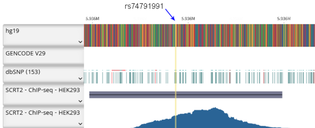
Figure S1. The region of rs74791991 showed a binding activity to the SCRT2 gene in HEK293 cells. Information were retrieved from the RegulomeDB.
