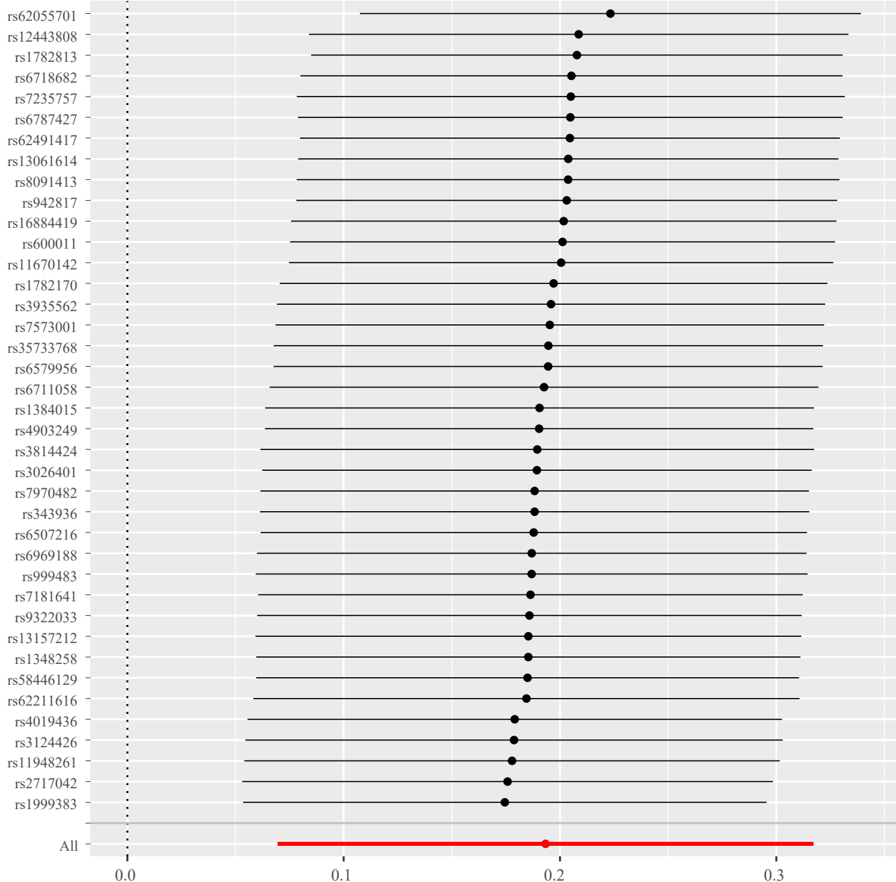
Supplementary Figure 1.2 MR leave-one-out sensitivity analysis for 'Irritability || id:ukb-b-13745' on 'Smoking status || id:ebi-a-GCST90029014'
