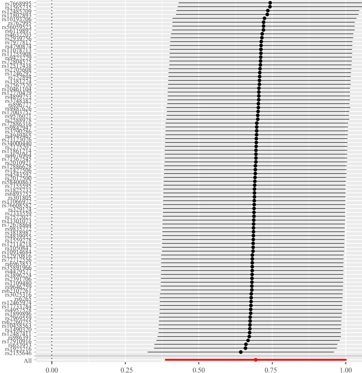
Supplementary Figure 1.1 MR leave-one-out sensitivity analysis for 'Smoking status || id:ebi-a-GCST90029014' on 'bipolar disorder || id:ieu-b-41'
