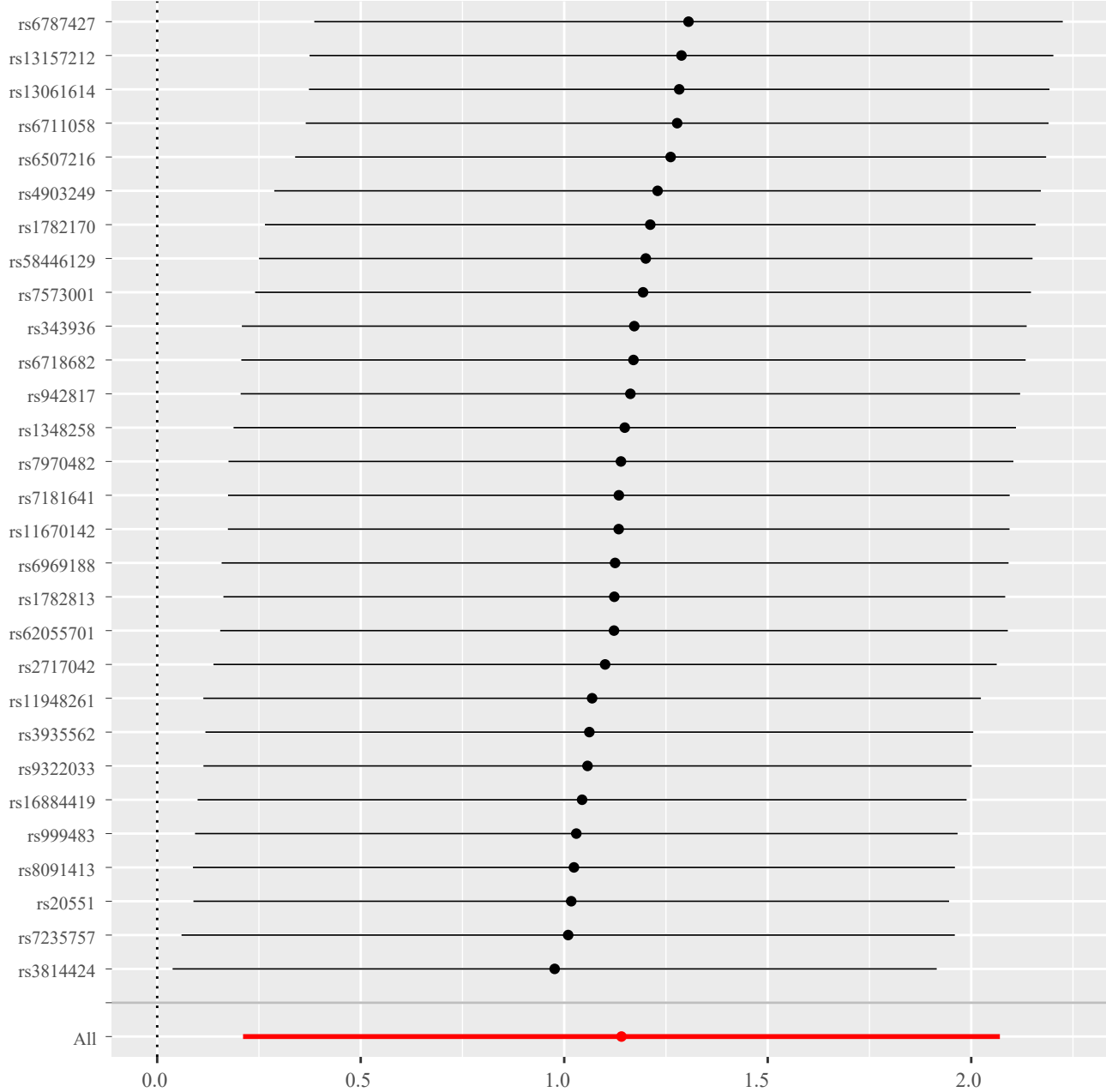
Supplementary Figure 1.3 MR leave-one-out sensitivity analysis for 'Irritability || id:ukb-b-13745' on 'bipolar disorder || id:ieu-b-41'
