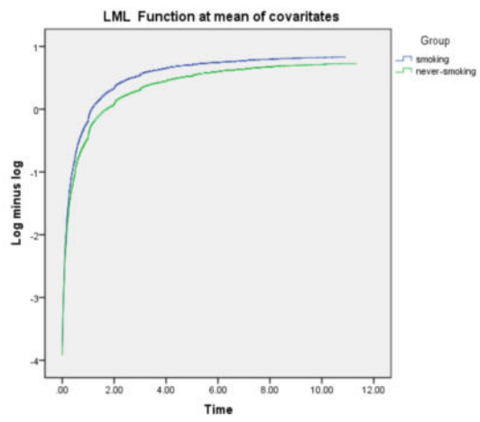
Supply Figure3 Plot to check proportional hazards assumption of the Cox model.
