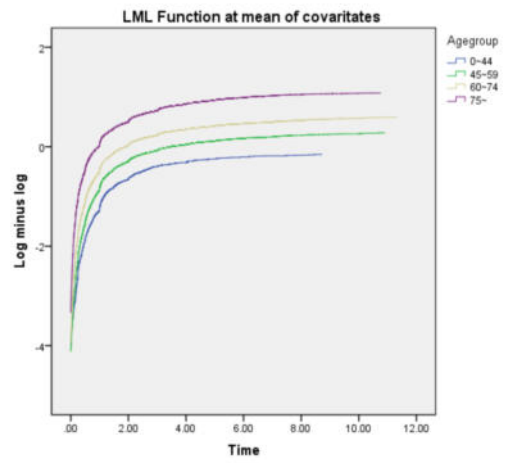
Supply Figure3 Plot to check proportional hazards assumption of the Cox model.
