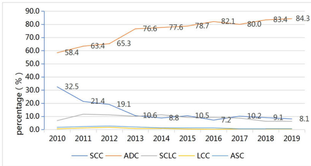
Supply Figure1 The percentages of histological subtypes of lung cancer from the year of 2010 to 2019
