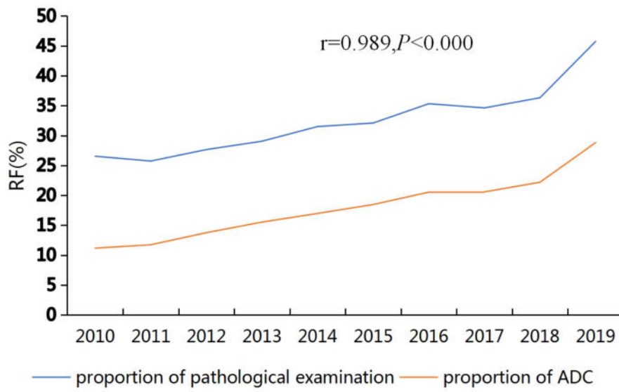
Supply figure2 The correlation of the proportion of pathological and the proportion of ADC of lung cancer
